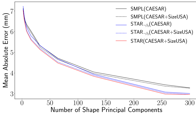
Fig. 4: Generalization Accuracy: Evaluating STAR and SMPL on unseen bodies. STAR -β 2 (CAESAR) is STAR trained on CAESAR with pose correctives depending on pose only (i.e. independent of β 2 ), STAR -β 2 (CAESAR+SizeUSA) is STAR trained on CAESAR and SizeUSA with pose corrective blend shapes depending on pose only, and STAR(CAESAR+SizeUSA) is STAR trained on CAESAR and SizeUSA with pose and shape dependent pose corrective blend shapes.
